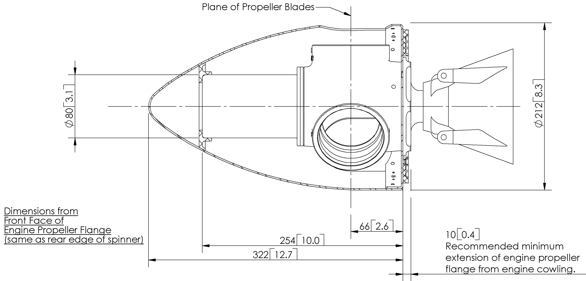
Principal Dimensions of AP332 Propeller with \phi 212\text{mm} (8.3in) Spinner (Example shown mounted on Rotax engine) Primary dimensions in millimeters [secondary dimensions in inches]
